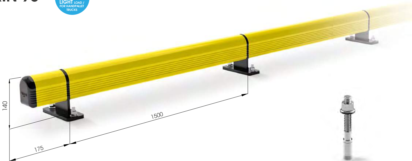
M12 GALVANISED STEEL
