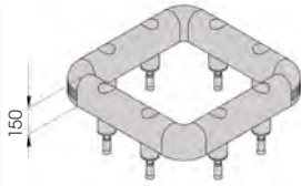
SF20 STAINLESS STEEL
