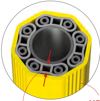
FLEXIBLE NEW ANTISHOCK BUMPER
